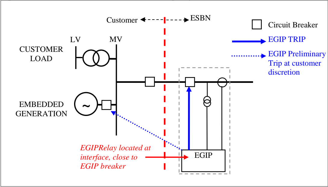
Figure 12: MV connected EG ≥2MVA installed capacity
